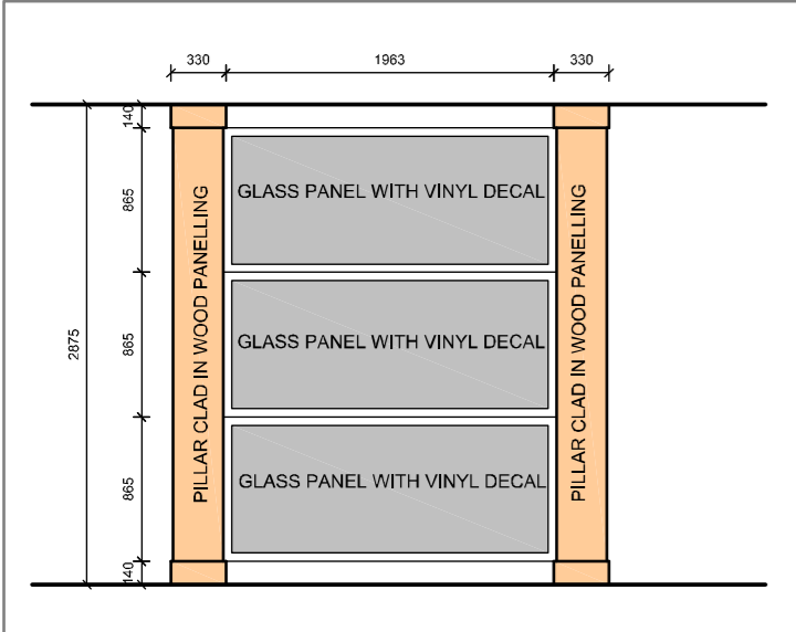
DECORATIVE PANEL DETAIL SCALE 1:50
